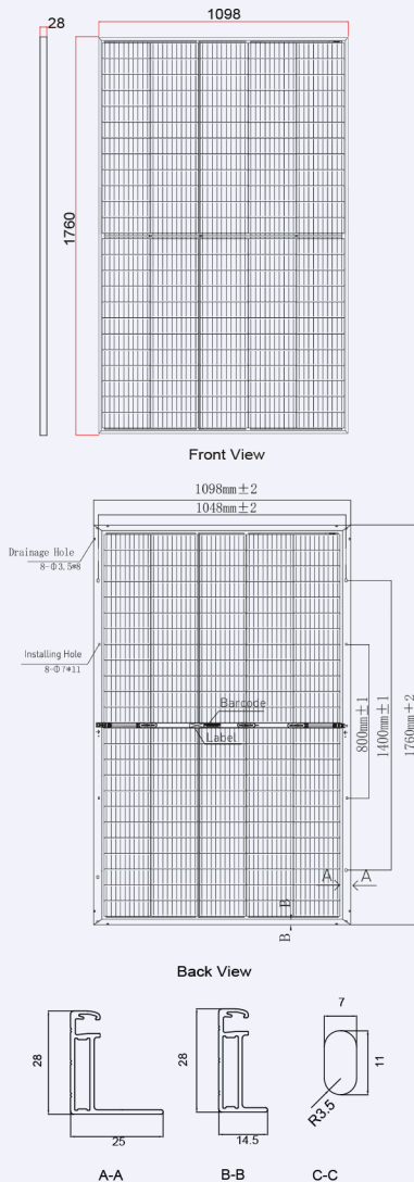
DIMENSIONS OF PV MODULE(mm)
